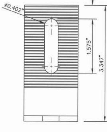
PART# 17661 – QB2 L-FOOT BRACKET. (304 SERIES STAINLESS STEEL).
